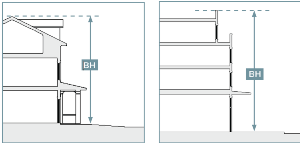
Figure 1: Graphic showing how to measure building height (BH) of a pitched-roof building (left) and a flat roofed building (right).
